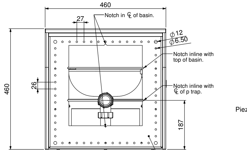
REAR VIEW
