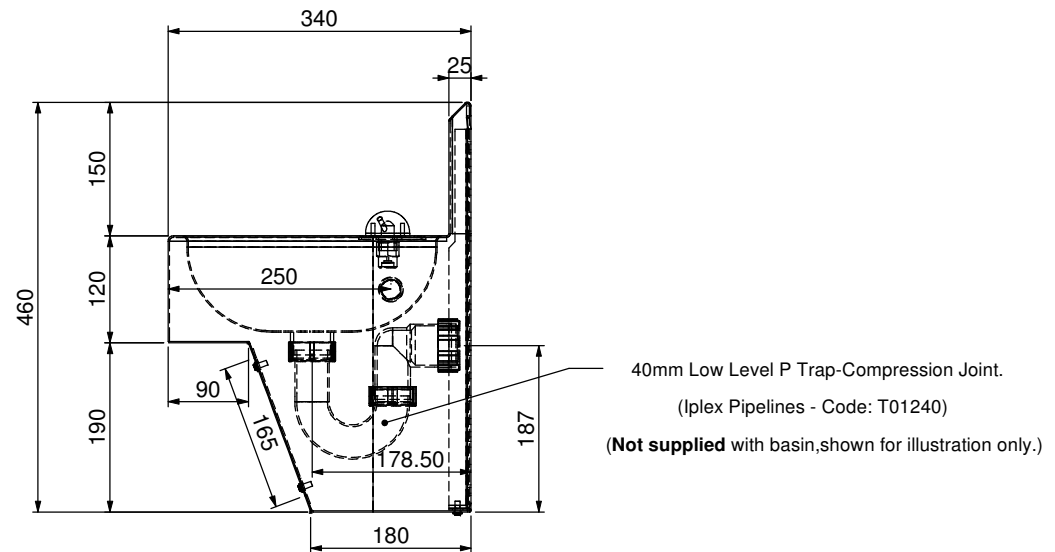
END VIEW
