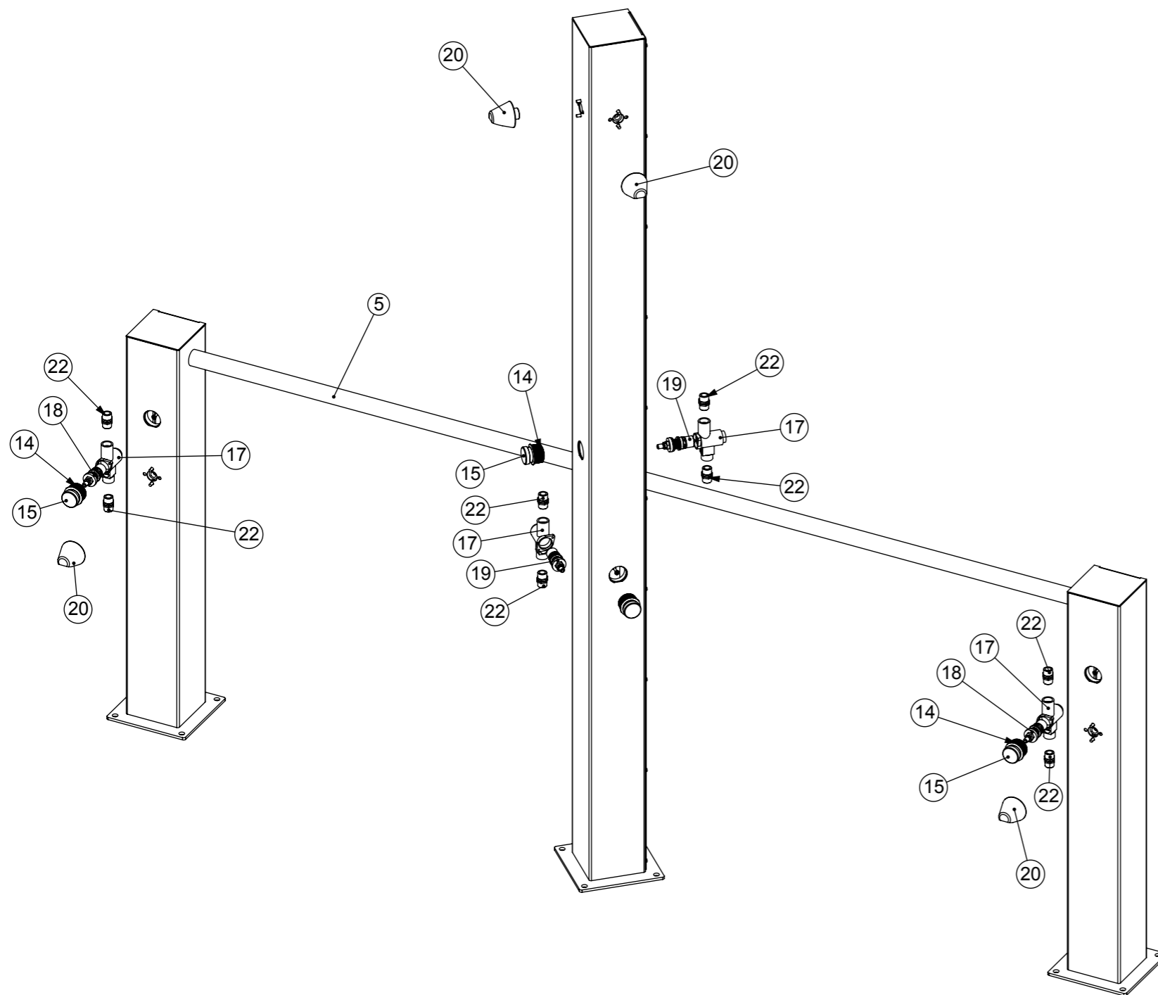
EXPLODED PARTS
