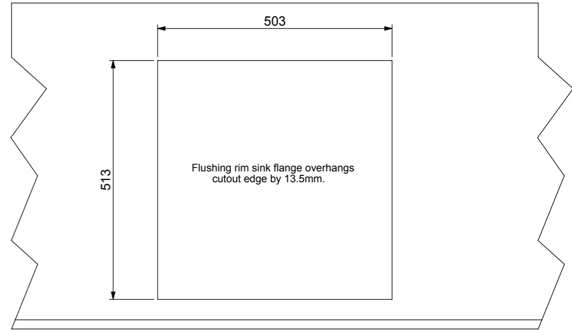
BENCHTOP CUTOUT SIZE
