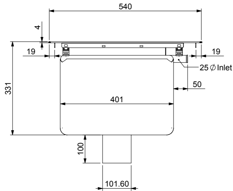
END VIEW
