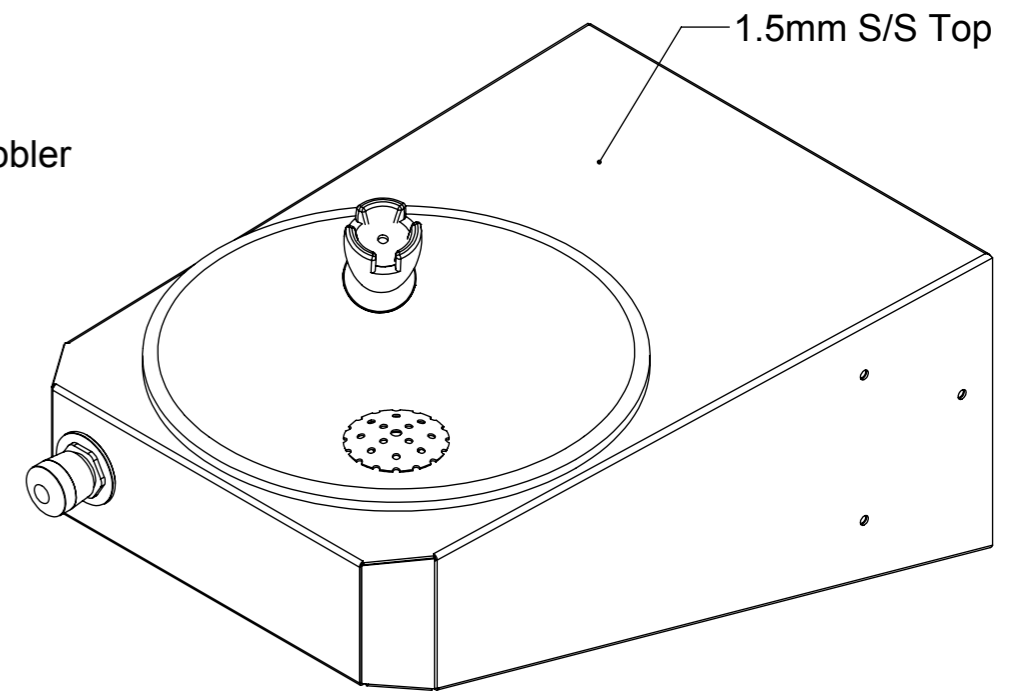
ISOMETRIC VIEW
