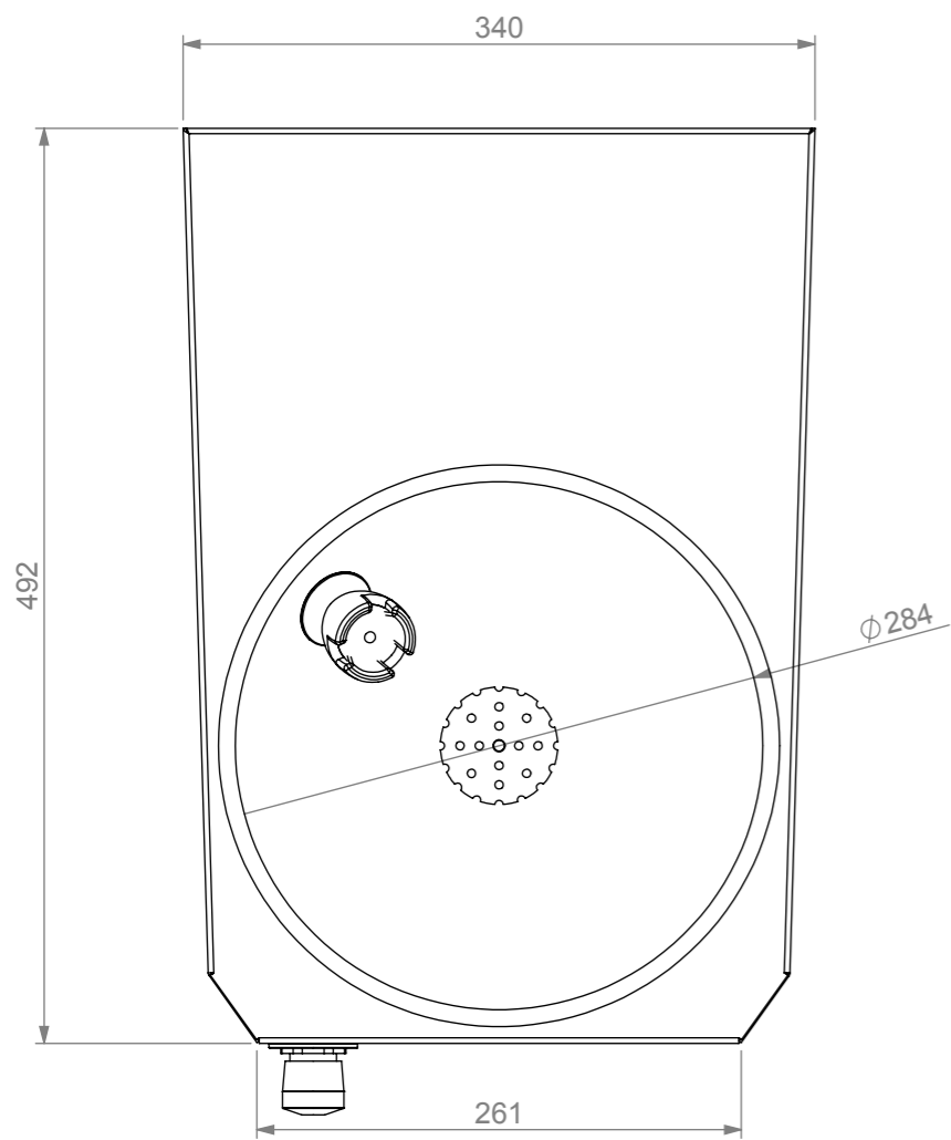
PLAN VIEW
