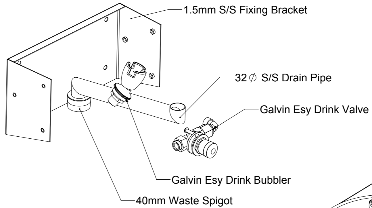
INTERNAL VIEW
