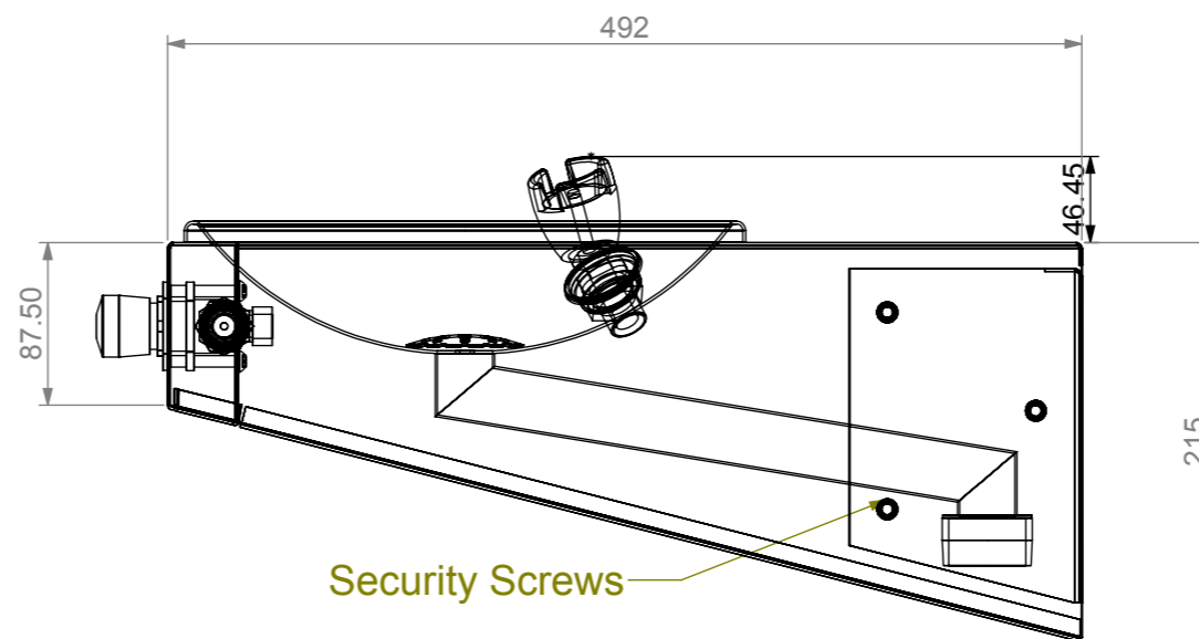
END VIEW
