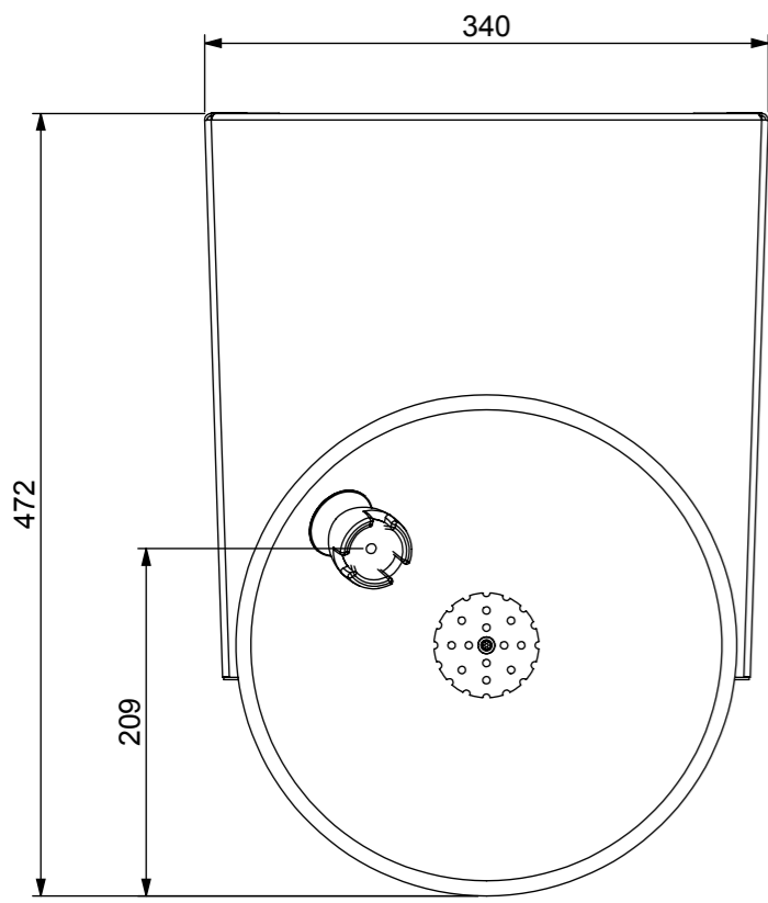
PLAN VIEW
