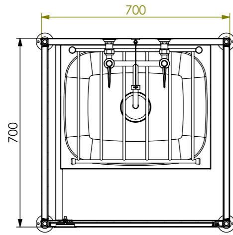
SECTION AO-AO
