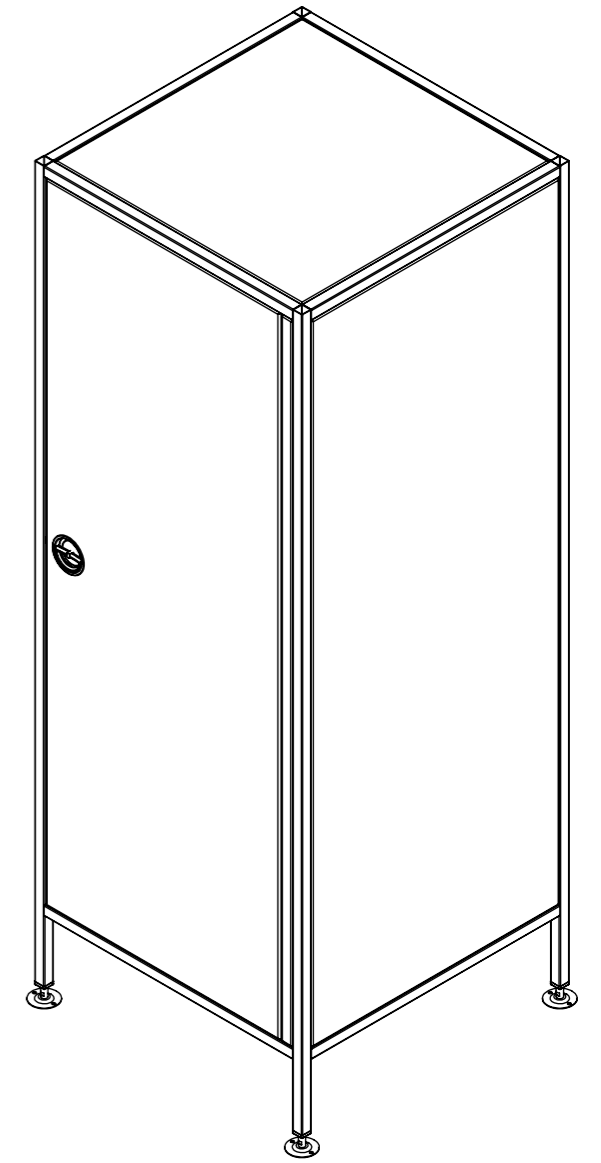
ISOMETRIC VIEW
