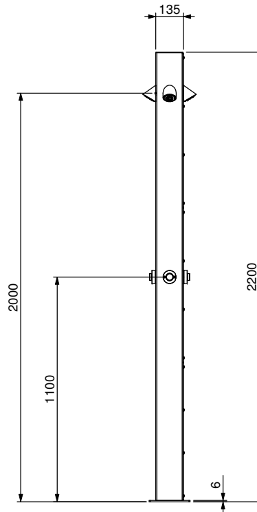
END VIEW
